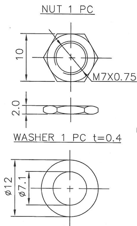
TERMINAL DETAIL
