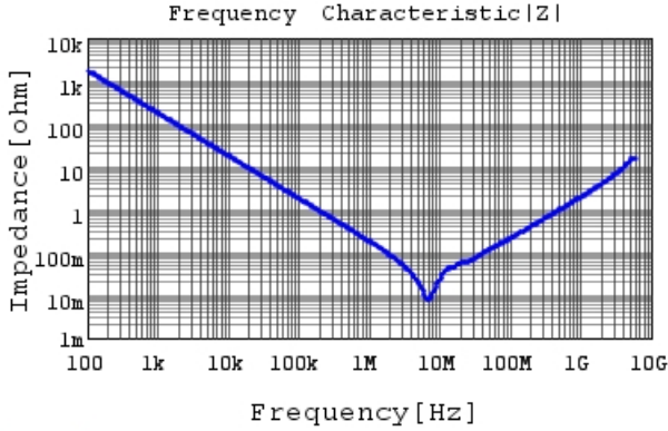
GRM219R71E105KA88 |Z| DC0V, 25degC
