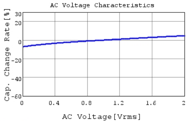
GRM219R71E105KA88 C-AC Voltage capchange, DC
