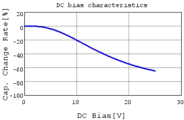
GRM219R71E105KA88 C-DC bias capchange, 25.0c
