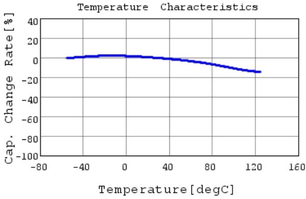
GRM219R71E105KA88 C-Temp. capchange, DC0.0V,
