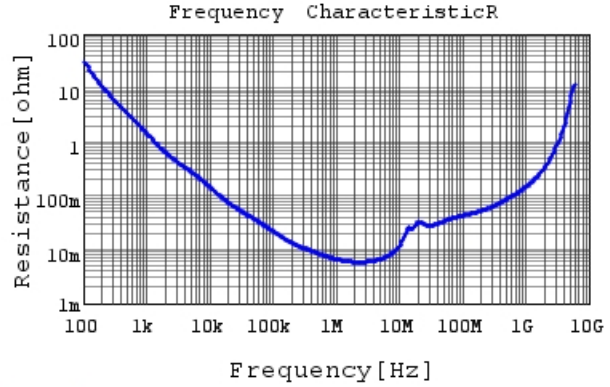
GRM219R71E105KA88 R DC0V, 25degC
