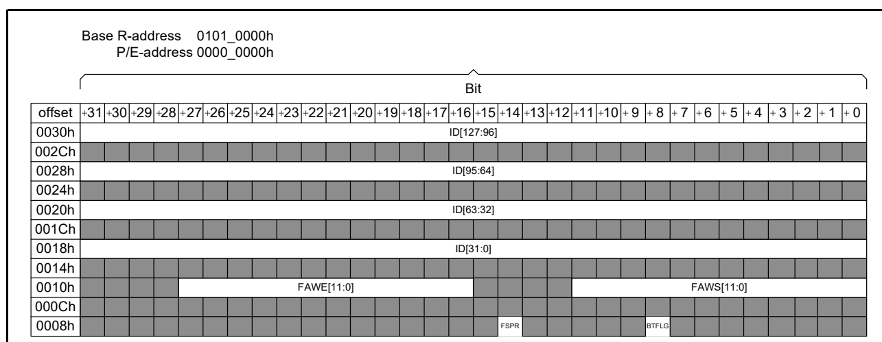
Figure 42.5 Configuration area bit map
