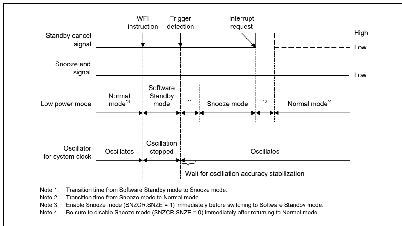
Figure 10.9 When interrupt request signal is generated in Snooze mode
