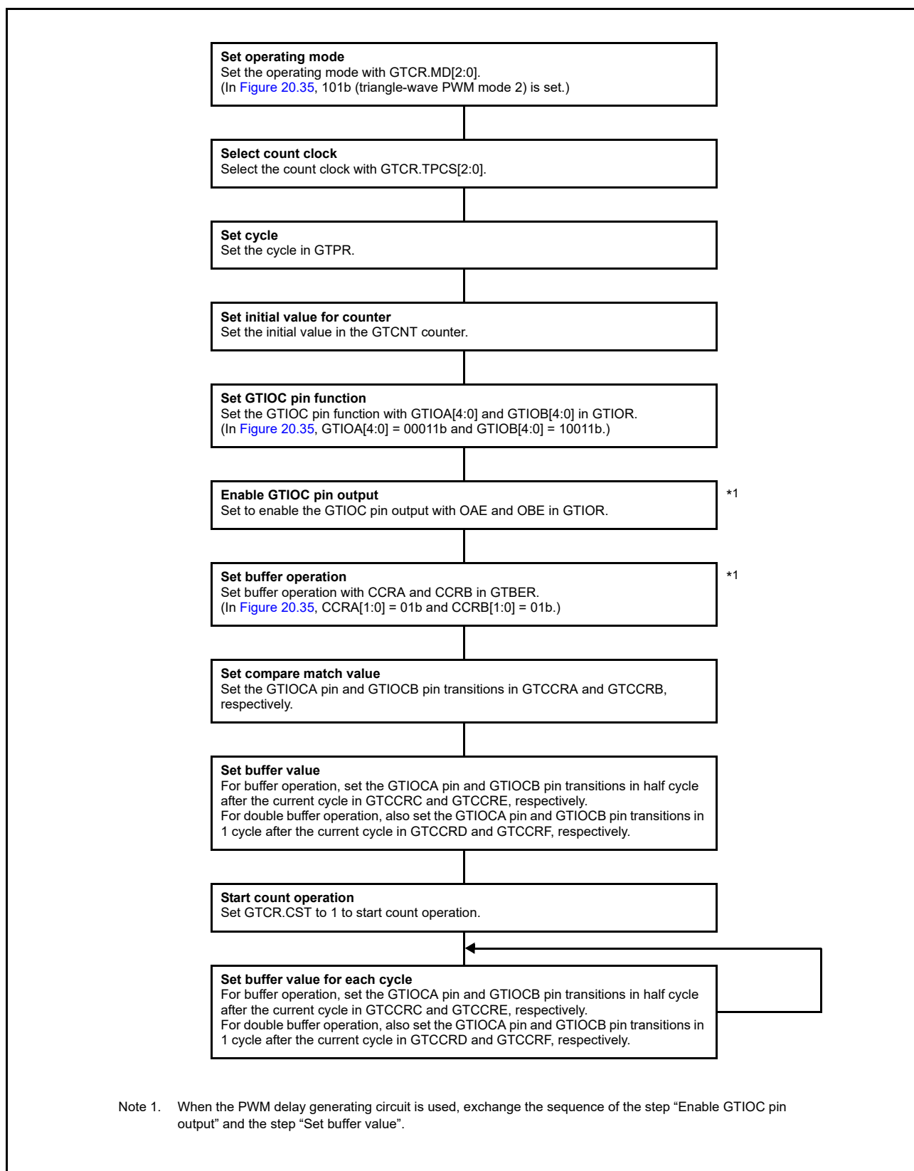
Figure 20.36 Example for setting triangle-wave PWM mode 2
