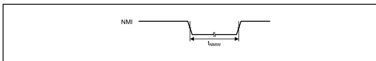
Figure 46.33 NMI interrupt input timing
