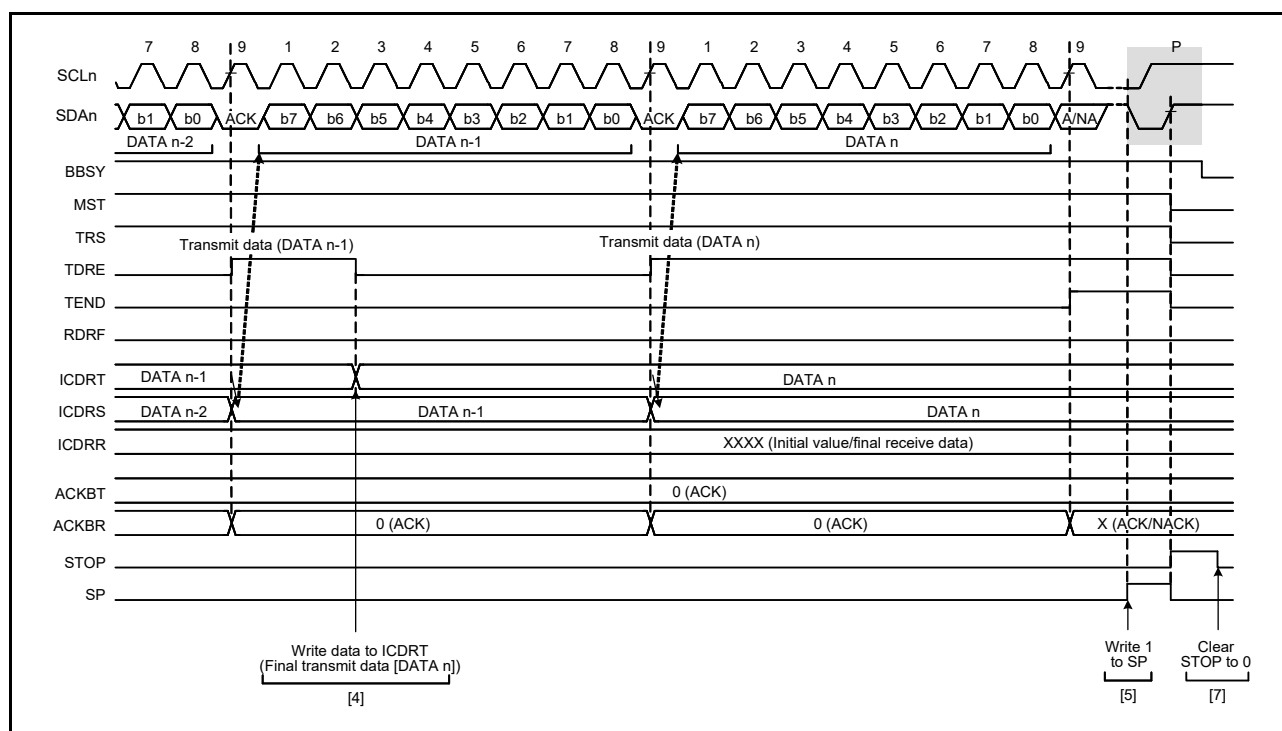
Figure 29.9 Master transmit operation timing (3)
