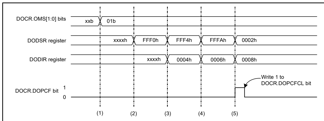
Figure 40.3 Example operation in data addition mode
