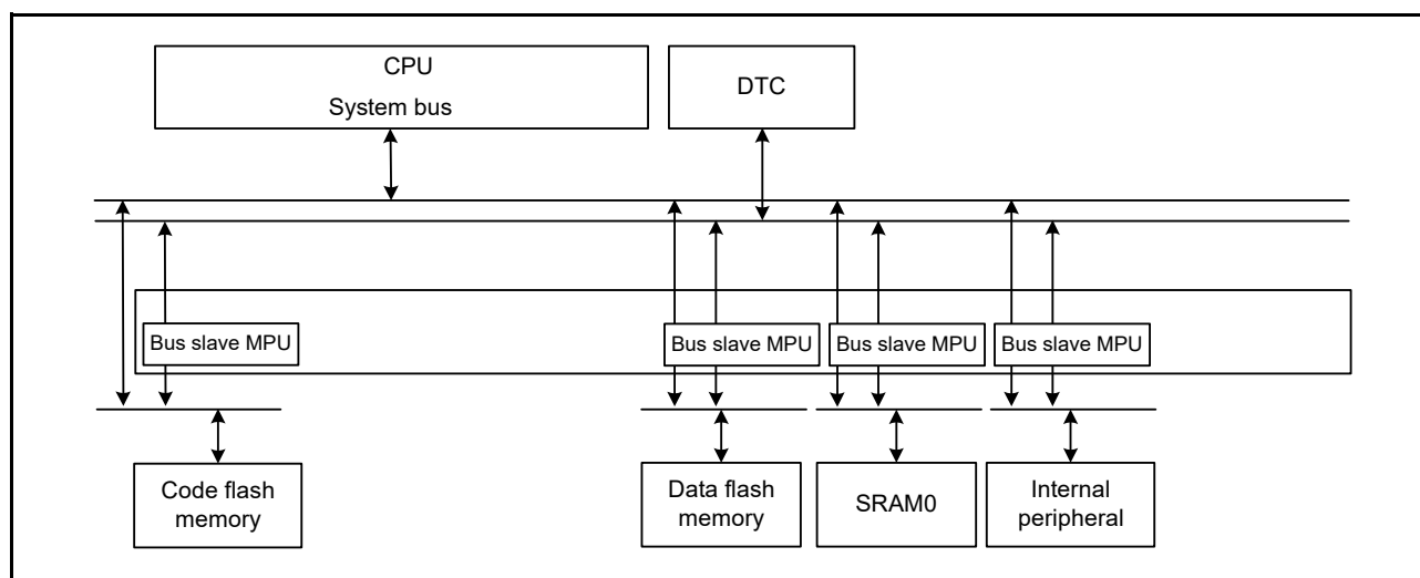
Figure 14.9 Bus slave MPU block diagram
