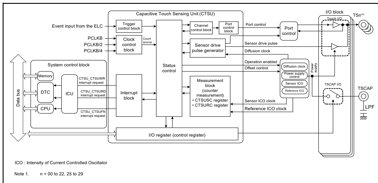
Figure 39.3 CTSU block diagram
