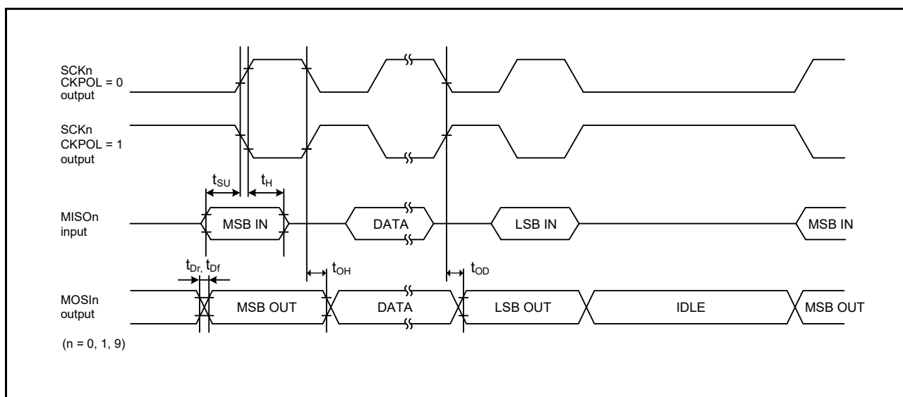
Figure 46.44 SCI simple SPI mode timing (master, CKPH = 1)
