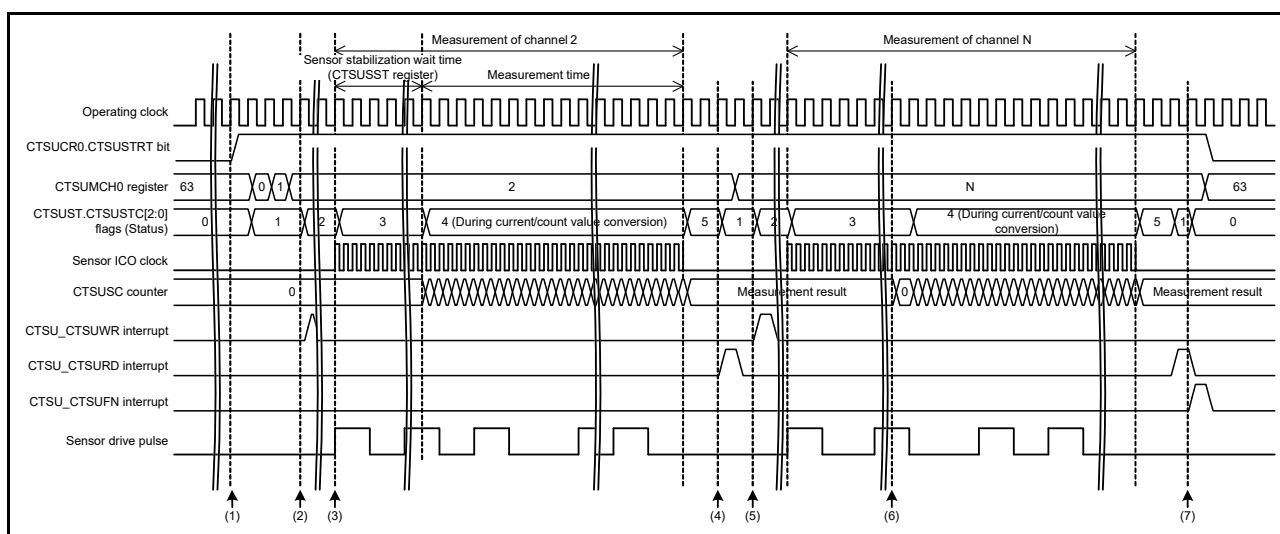
Figure 39.15 Timing of self-capacitance multi-scan mode when the measurement start condition is a software trigger
