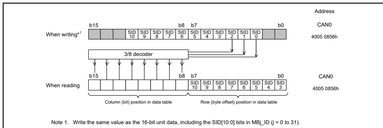
Figure 30.5 Writes to and reads from AFSR
