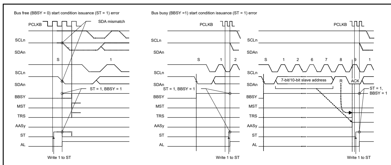
Figure 29.42 Arbitration-lost when start condition is issued (MALE = 1)
