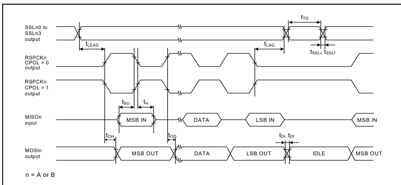
Figure 46.52 SPI timing (master, CPHA = 1) (bit rate: PCLKB division ratio is set to any value other than 1/2)
