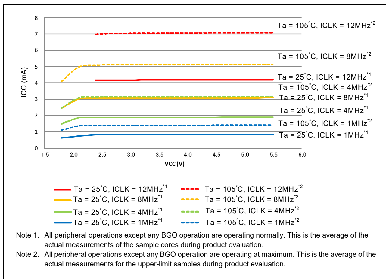
Figure 46.18 Voltage dependency in middle-speed mode (reference data)
