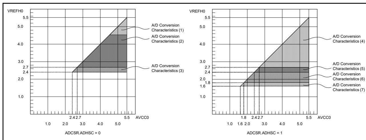
Figure 46.61 AVCC0 to VREFH0 voltage range
