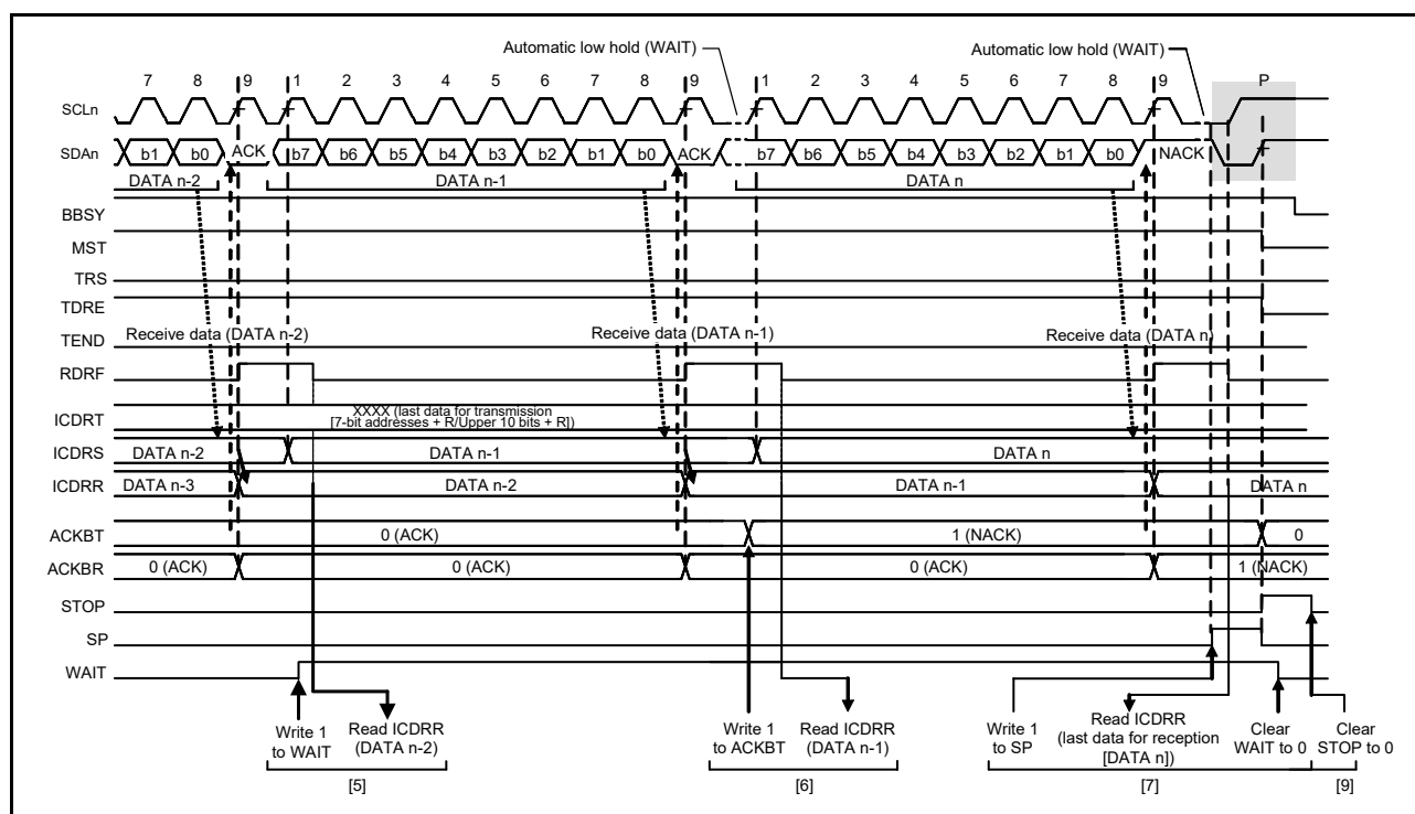
Figure 29.14 Master receive operation timing (3) when RDRFS = 0
