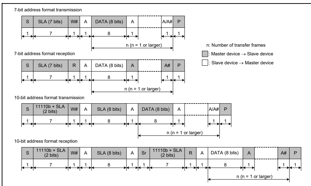
Figure 27.58 I 2 C bus format
