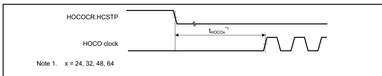
Figure 46.27 HOCO clock oscillator start timing (started by setting the HOCOCR.HCSTP bit)
