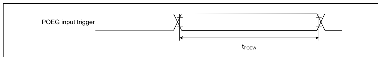
Figure 46.36 POEG input trigger timing
