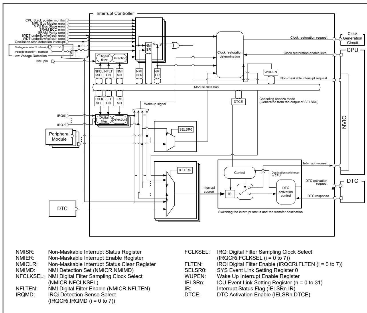
Figure 12.1 ICU block diagram
