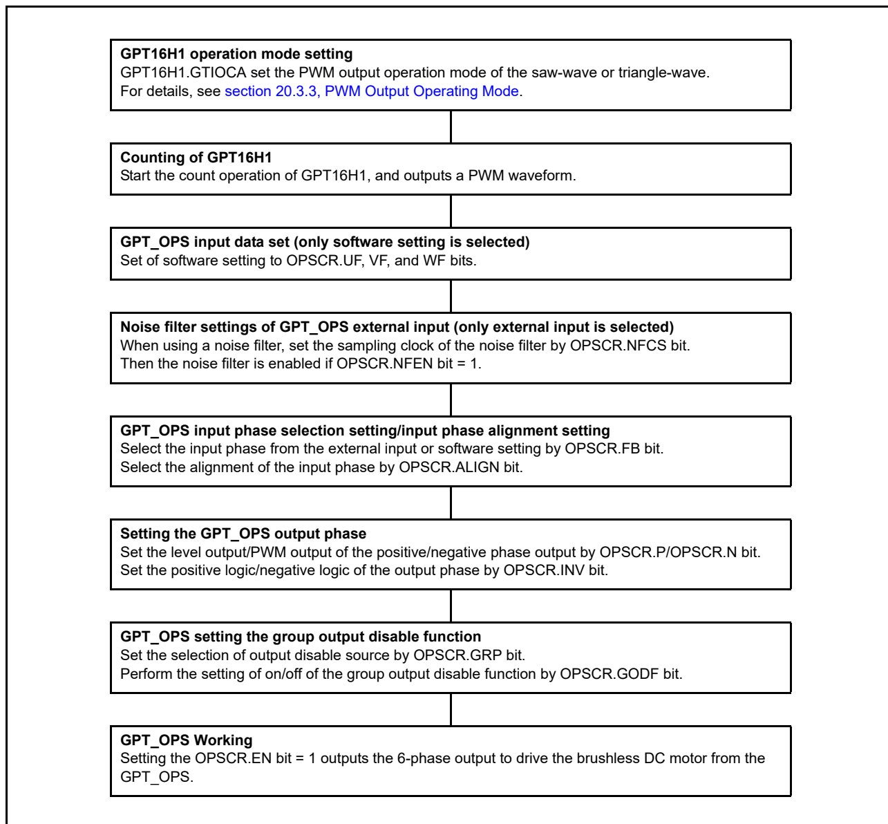
Figure 20.81 Example for setting of GPT_OPS start operation
