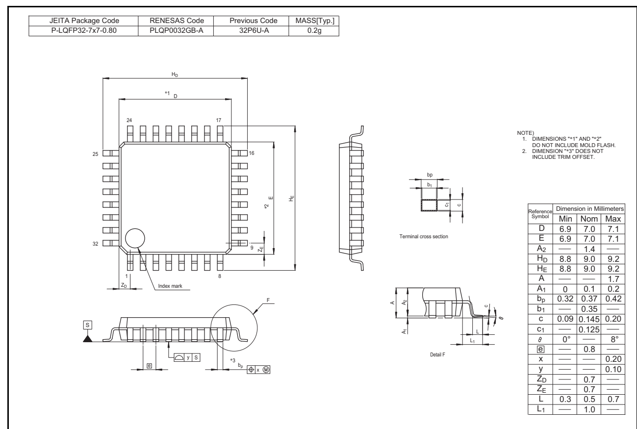
Figure 2.3 LQFP 32-pin
