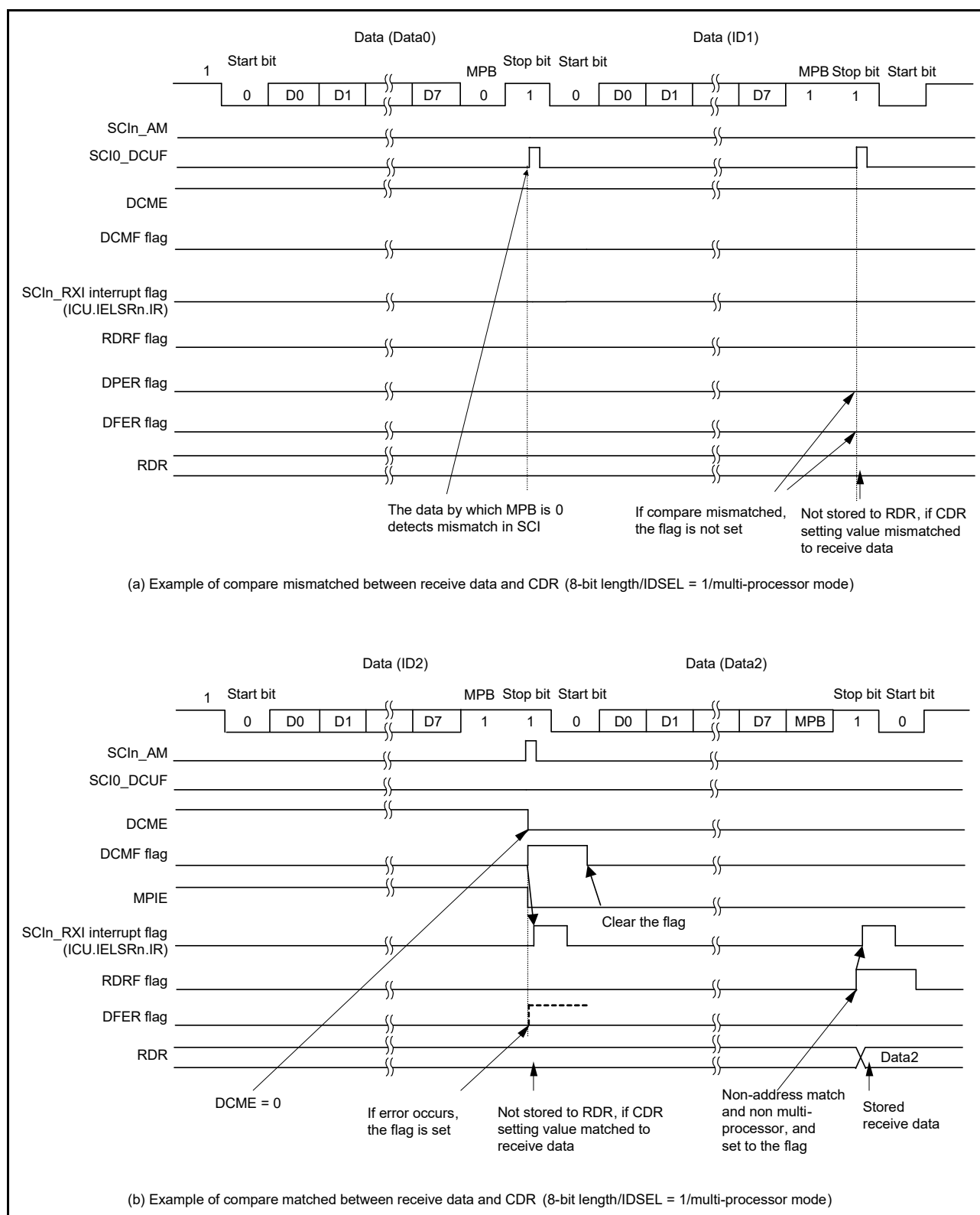
Figure 27.6 Example of address match (2) multi-processor mode
