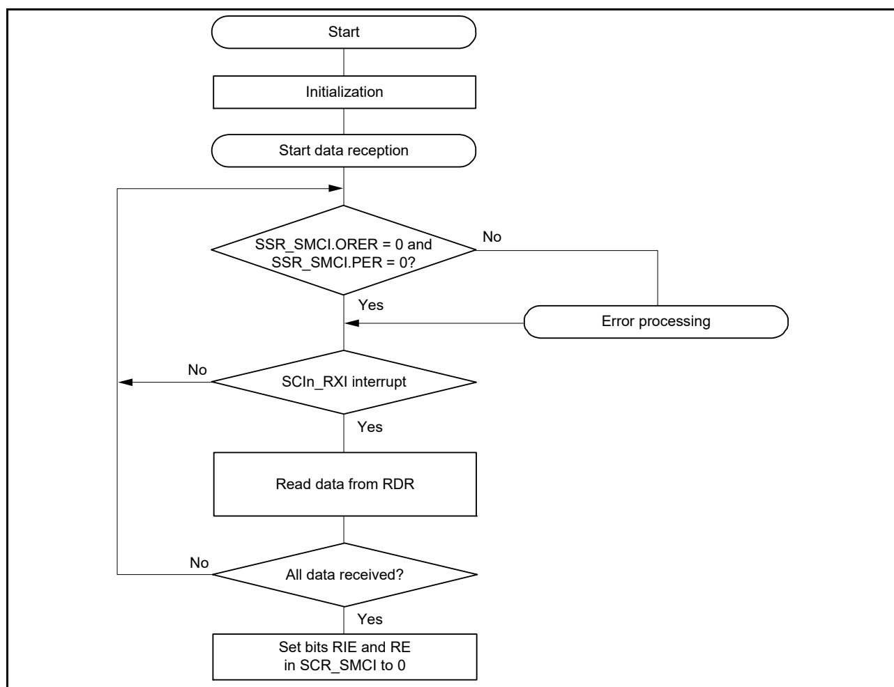
Figure 27.56 Example flow for smart card interface reception
