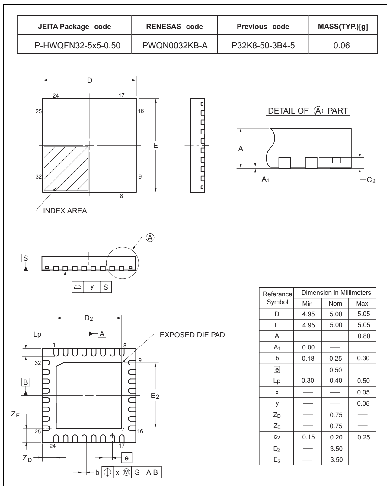
Figure 2.6 QFN 32-pin
