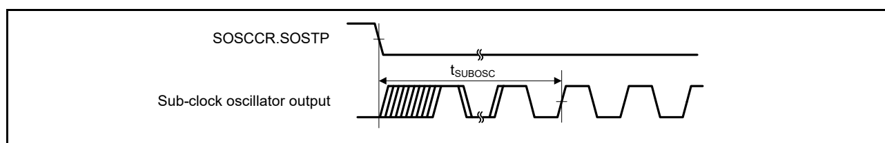
Figure 46.28 Sub-clock oscillation start timing
