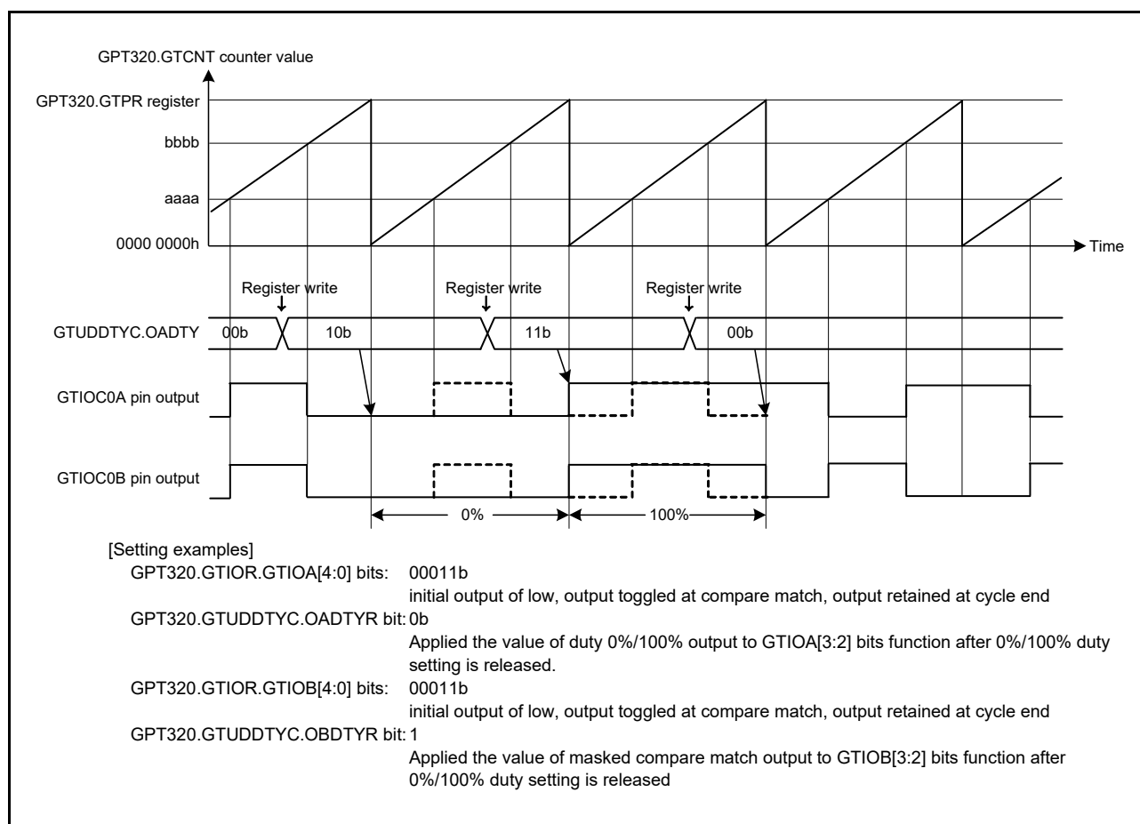
Figure 20.46 Example of output duty 0% and 100% function
