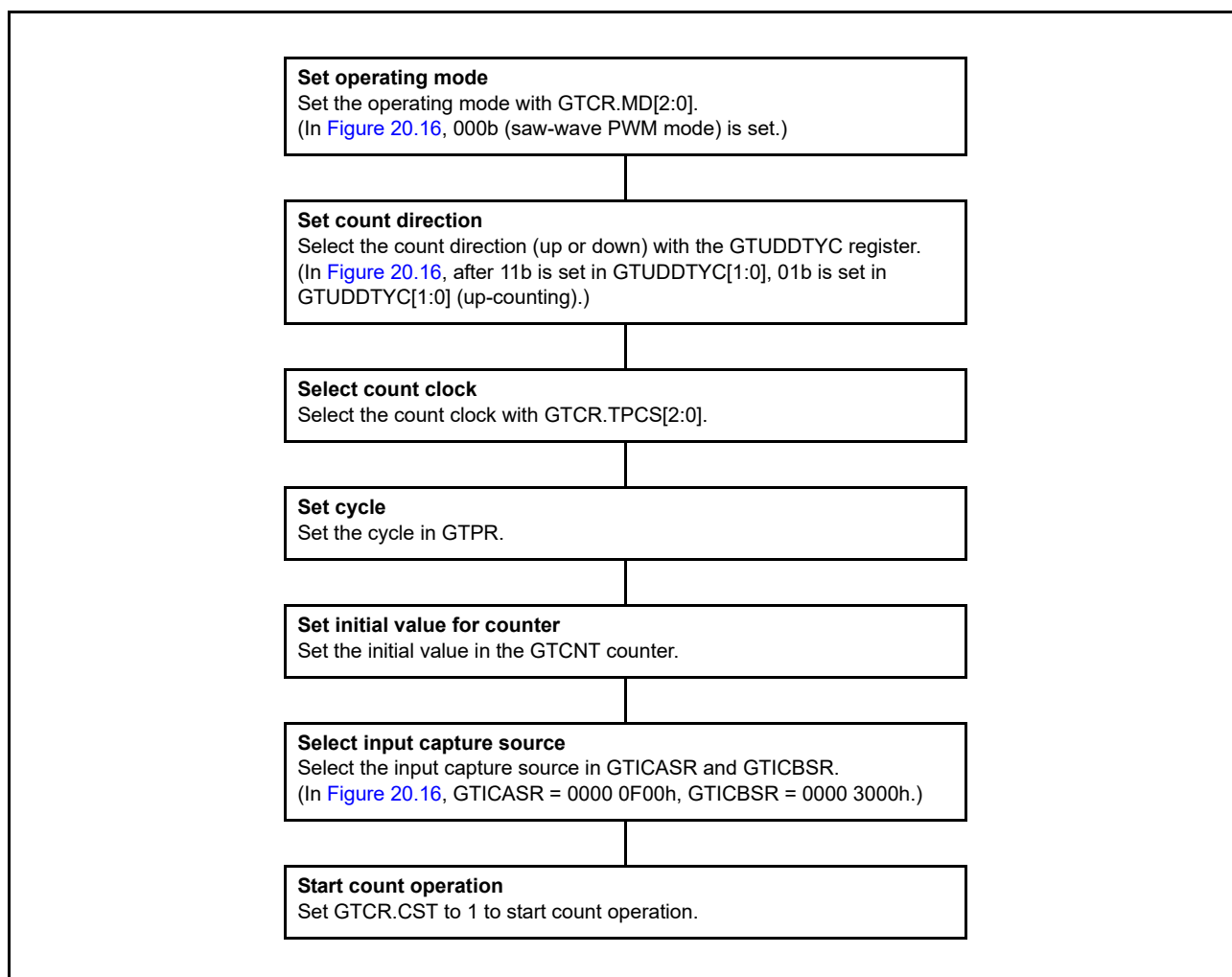
Figure 20.17 Example for setting input capture operation
