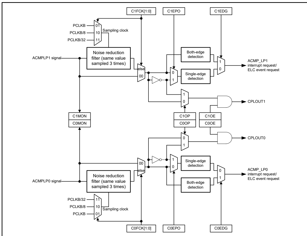
Figure 38.5 Noise filter and edge detection configuration
