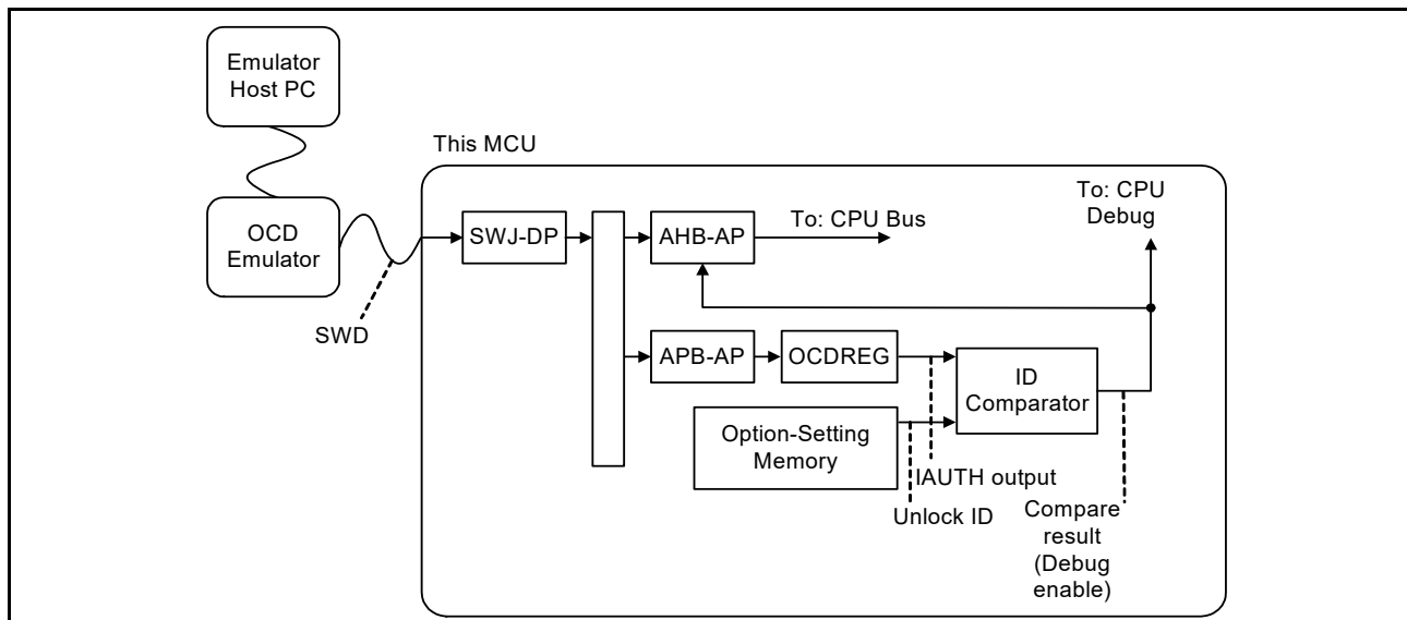
Figure 2.3 Authentication mechanism block diagram
