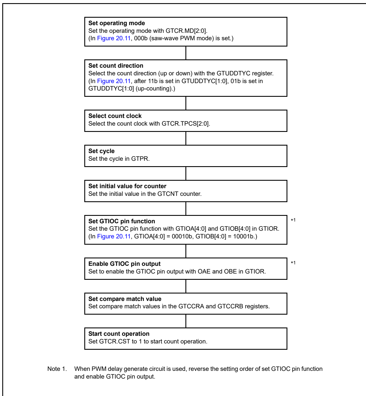
Figure 20.12 Example for setting low output and high output operation
