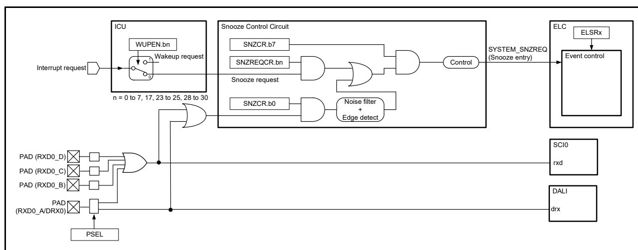
Figure 10.8 Snooze mode entry configuration
