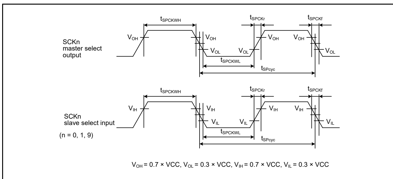
Figure 46.43 SCI simple SPI mode clock timing
