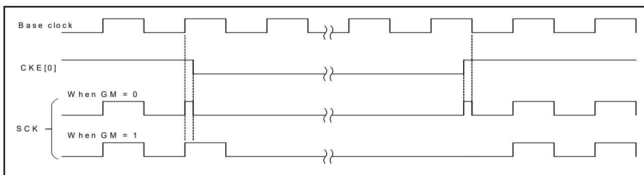
Figure 27.57 Clock output control
