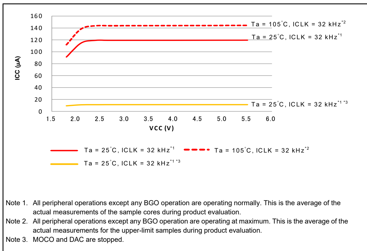
Figure 46.21 Voltage dependency in subosc-speed mode (reference data)
