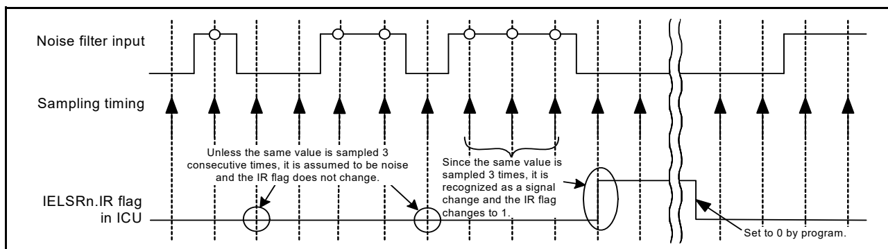
Figure 38.6 Noise filter and interrupt operation example
