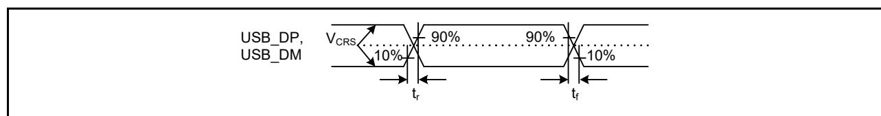
Figure 46.58 USB_DP and USB_DM output timing
