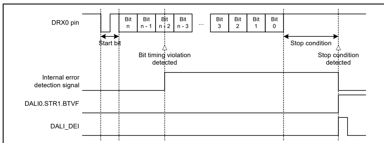
Figure 28.9 Bit timing violation error
