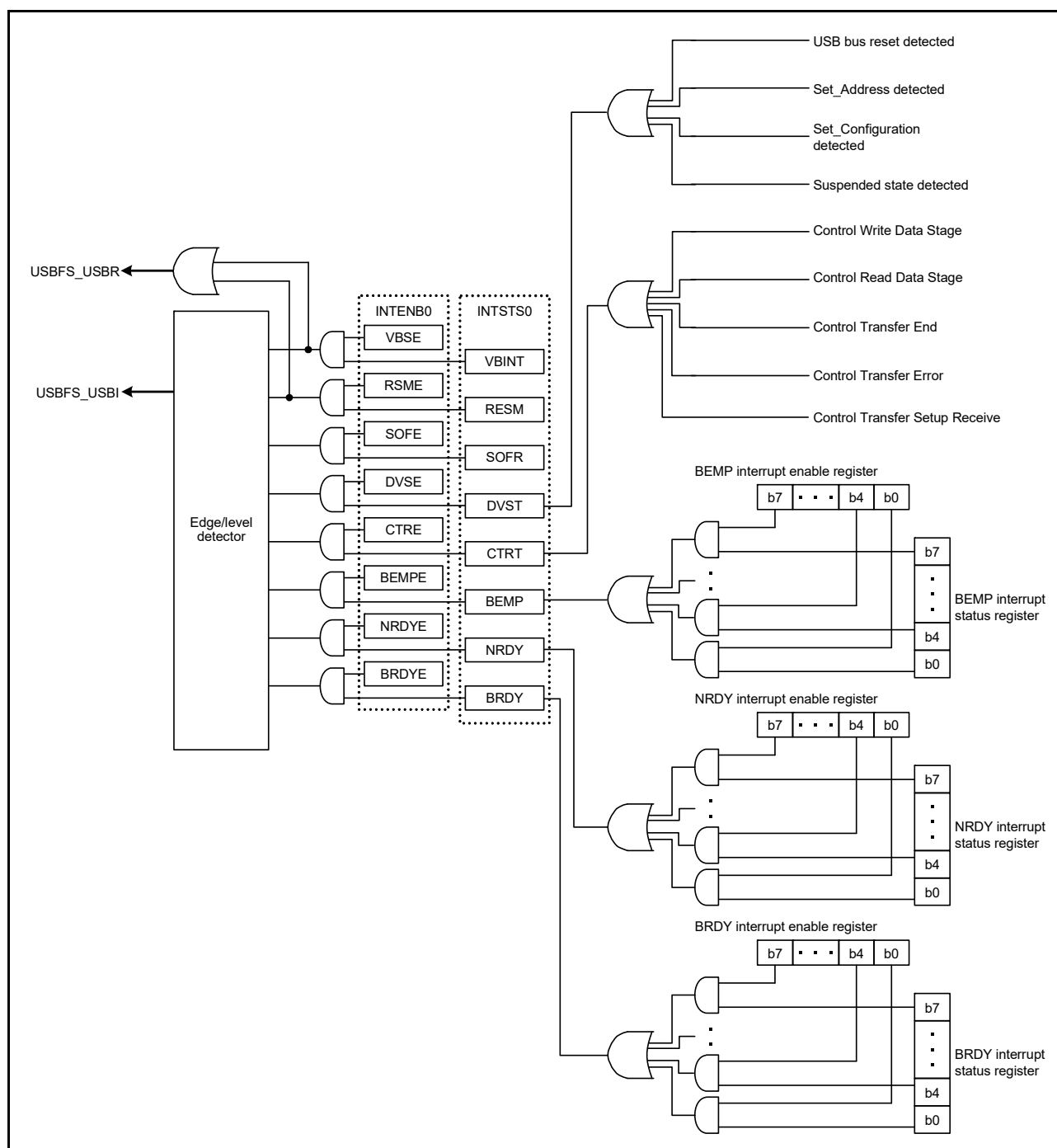
Figure 26.9 Circuits related to interrupts in USBFS
