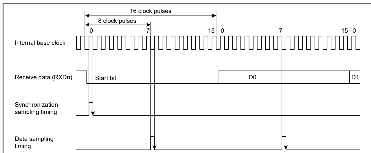
Figure 27.3 Receive data sampling timing in asynchronous mode
