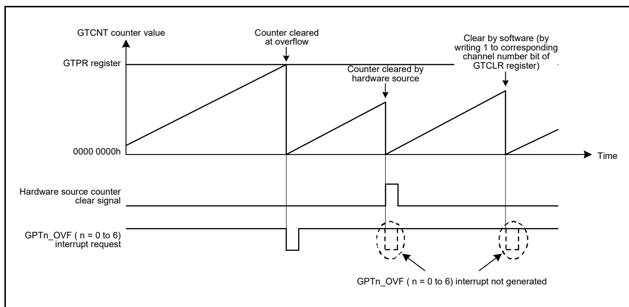
Figure 20.56 Relationship between counter clearing by hardware source and GPTn_OVF (n = 0 to 6) interrupt
