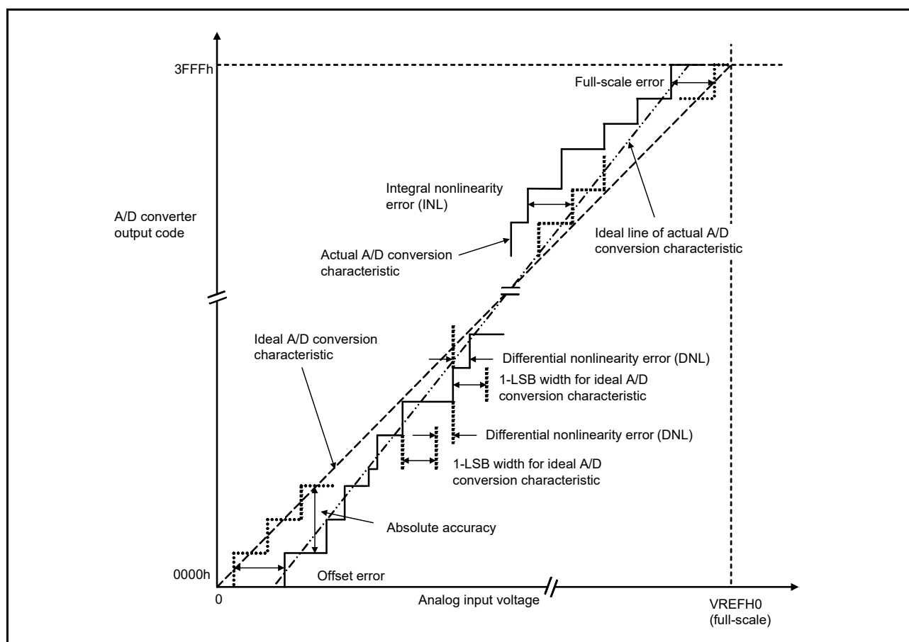
Figure 46.63 Illustration of 14-bit A/D converter characteristic terms
