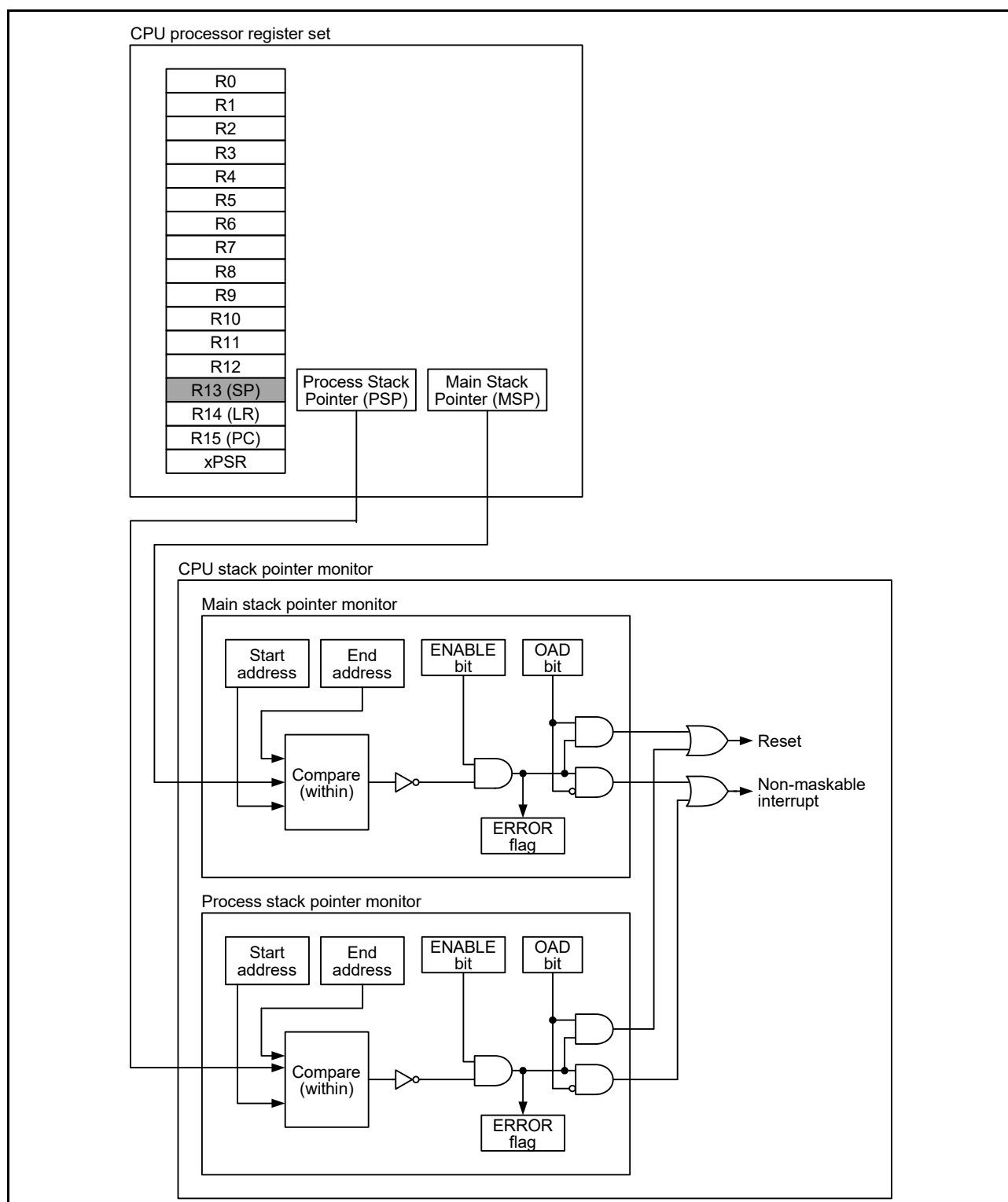
Figure 14.1 CPU stack pointer monitor block diagram
