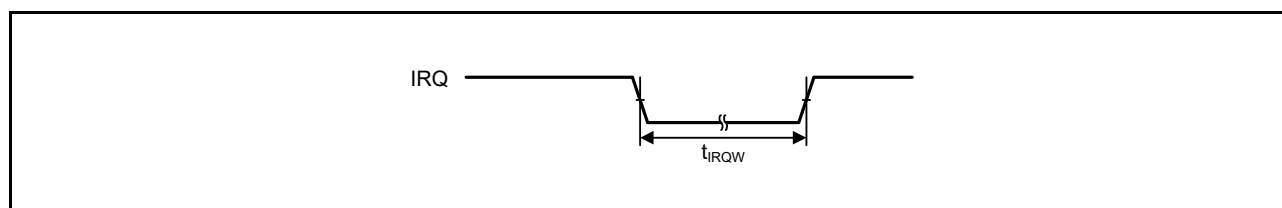
Figure 46.34 IRQ interrupt input timing
