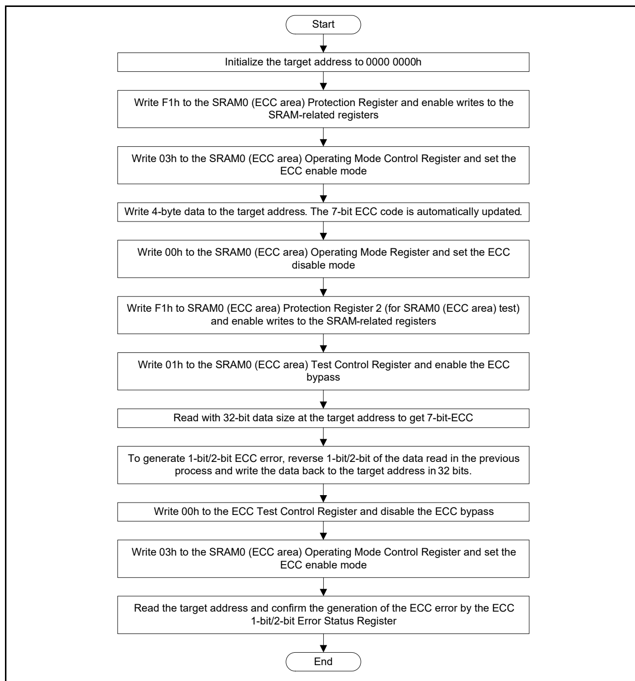
Figure 41.1 ECC decoder testing
