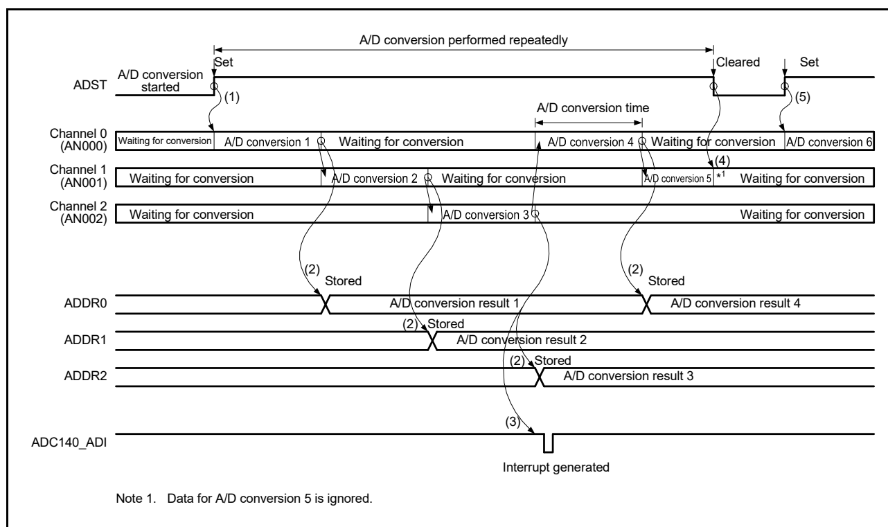
Figure 33.11 Example basic operation in continuous scan mode when AN000 to AN002 are selected
