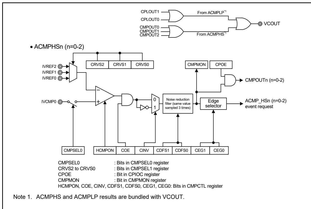
Figure 37.1 ACMPHS block diagram
