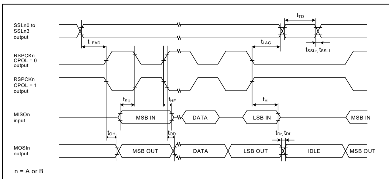
Figure 46.53 SPI timing (master, CPHA = 1) (bit rate: PCLKB division ratio is set to 1/2)
