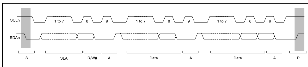
Figure 29.4 I 2 C bus timing (SLA = 7 bits)
