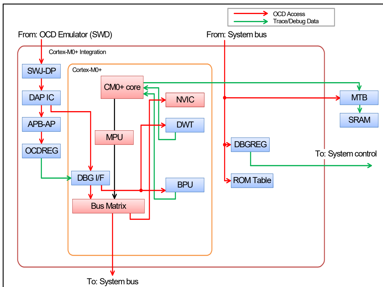
Figure 2.1 Cortex-M0+ block diagram
