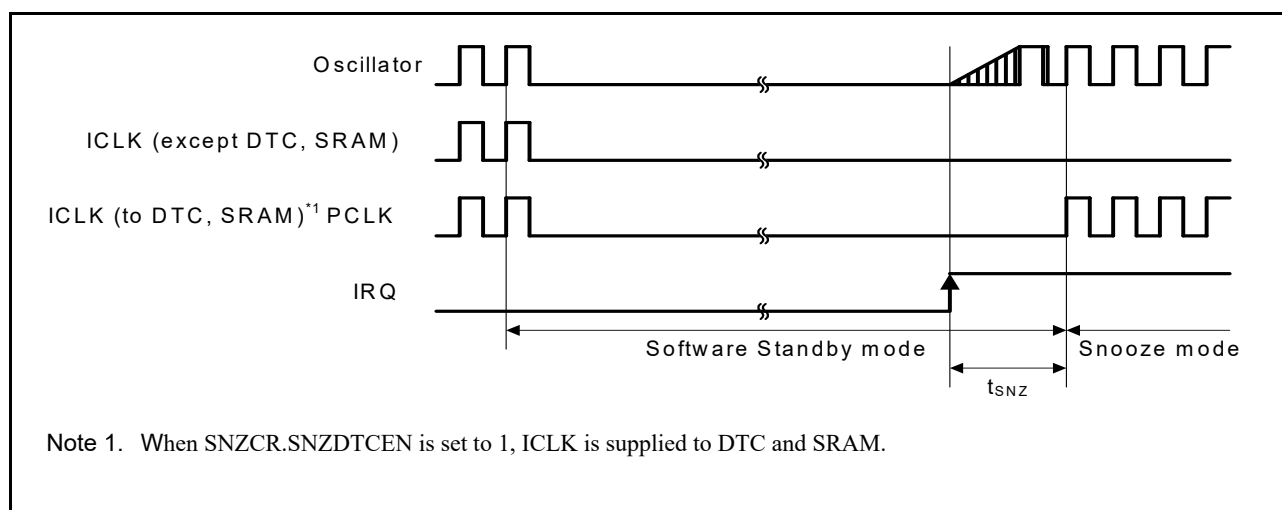
Figure 46.32 Recovery timing from Software Standby mode to Snooze mode
