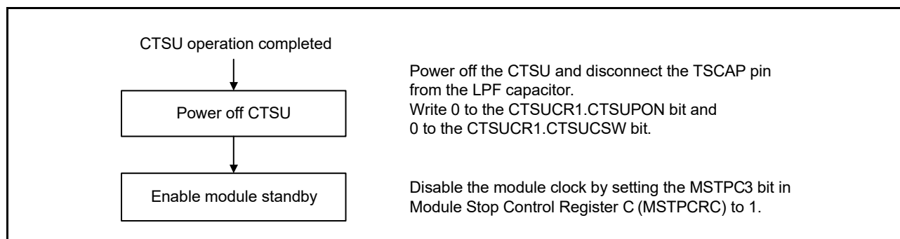
Figure 39.10 CTSU stopping flow
