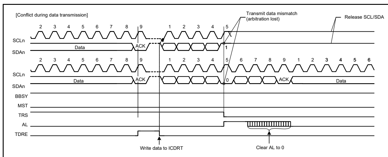
Figure 29.44 Example of slave arbitration-lost detection (SALE = 1)
