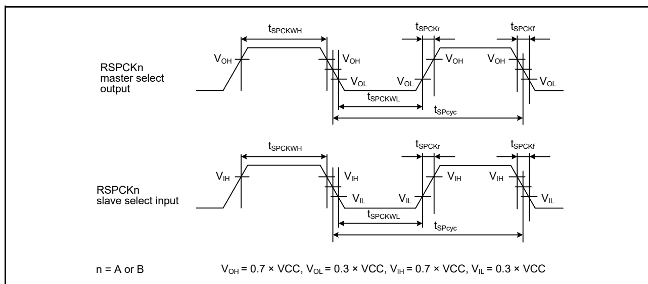
Figure 46.49 SPI clock timing
