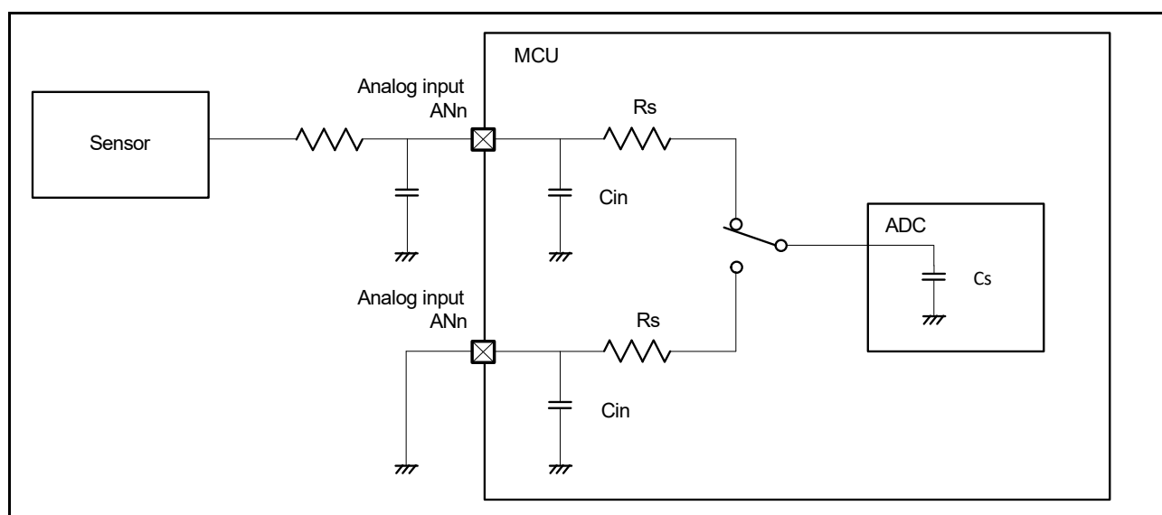
Figure 46.62 Equivalent circuit for analog input
