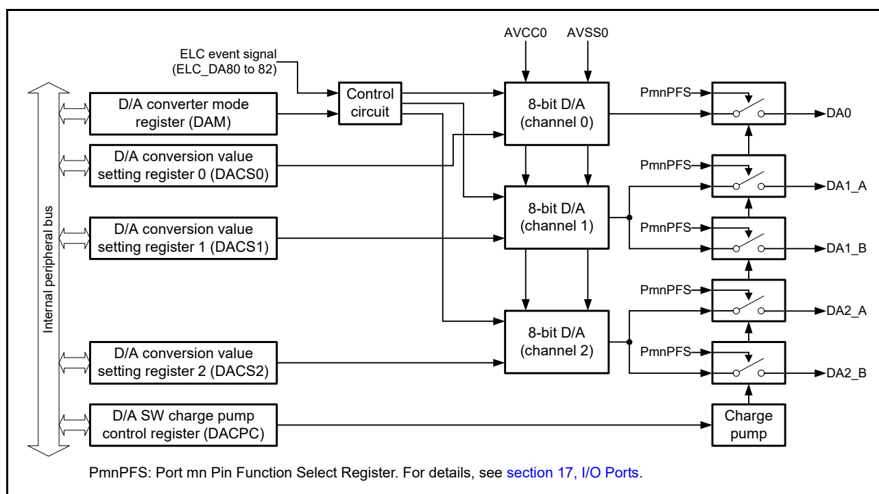
Figure 34.1 DAC8 block diagram
