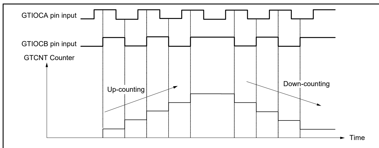
Figure 20.74 Example of phase counting mode 4
