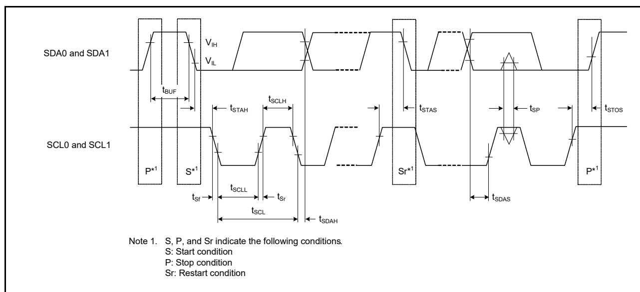
Figure 46.56 I²C bus interface input/output timing
