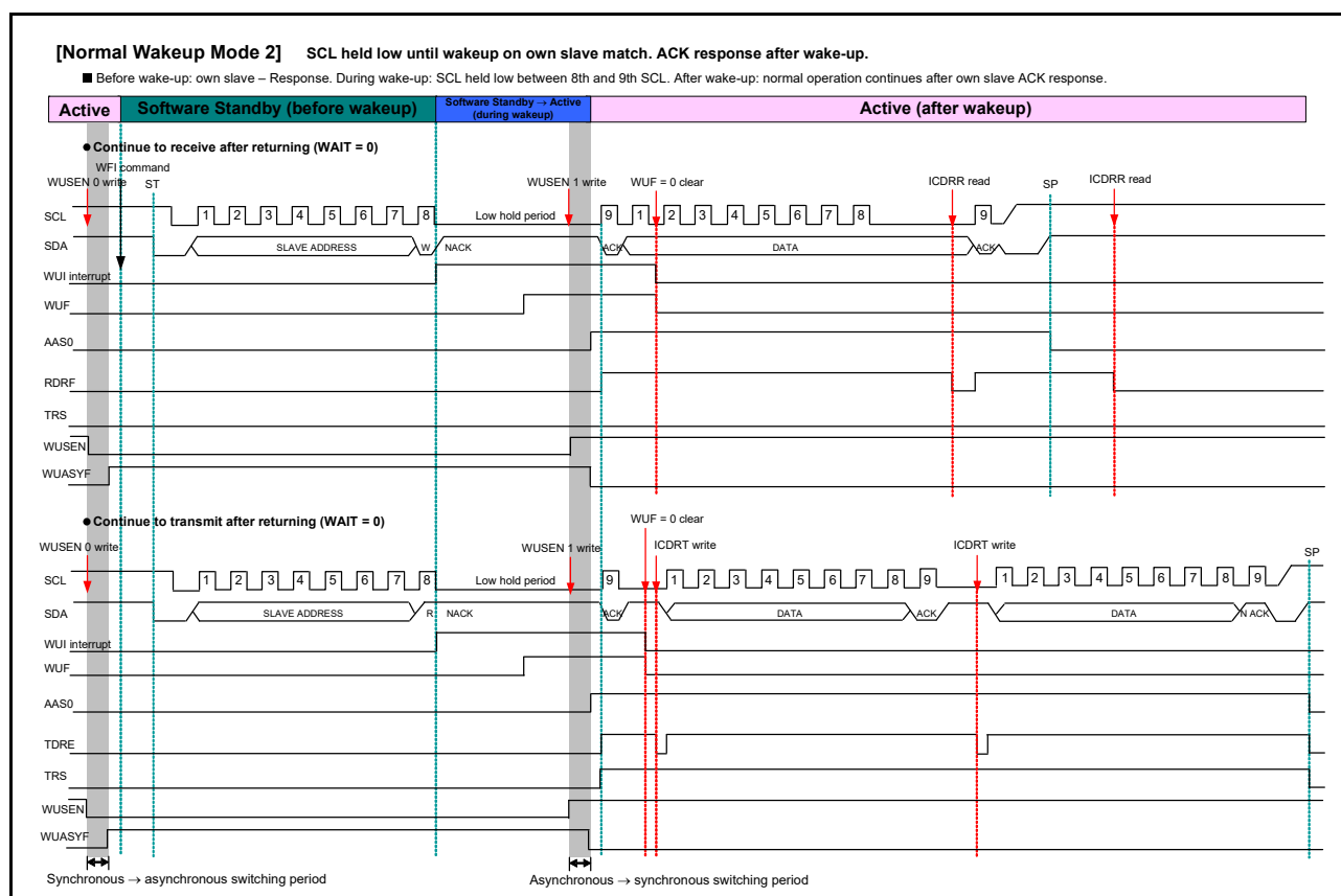
Figure 29.34 Timing of normal wakeup mode 2
