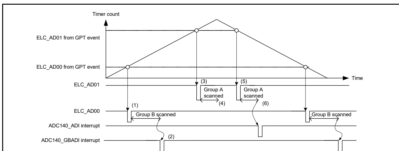
Figure 33.14 Example of operation in group scan mode with double trigger mode using synchronous triggers from the ELC
