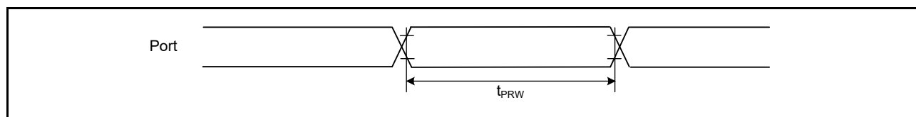
Figure 46.35 I/O ports input timing
