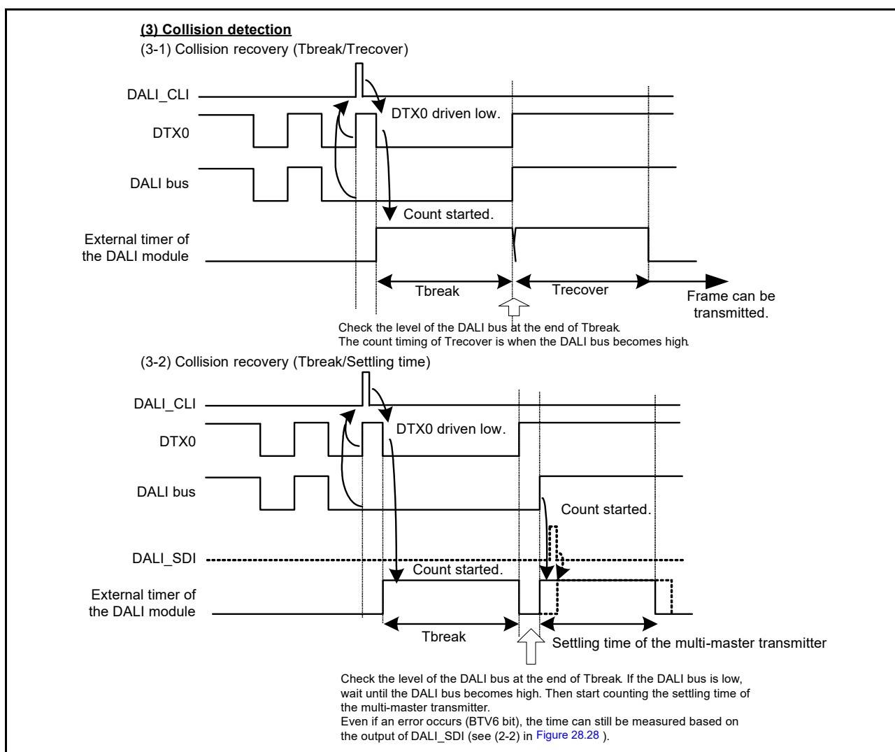
Figure 28.29 Example of collision detection
