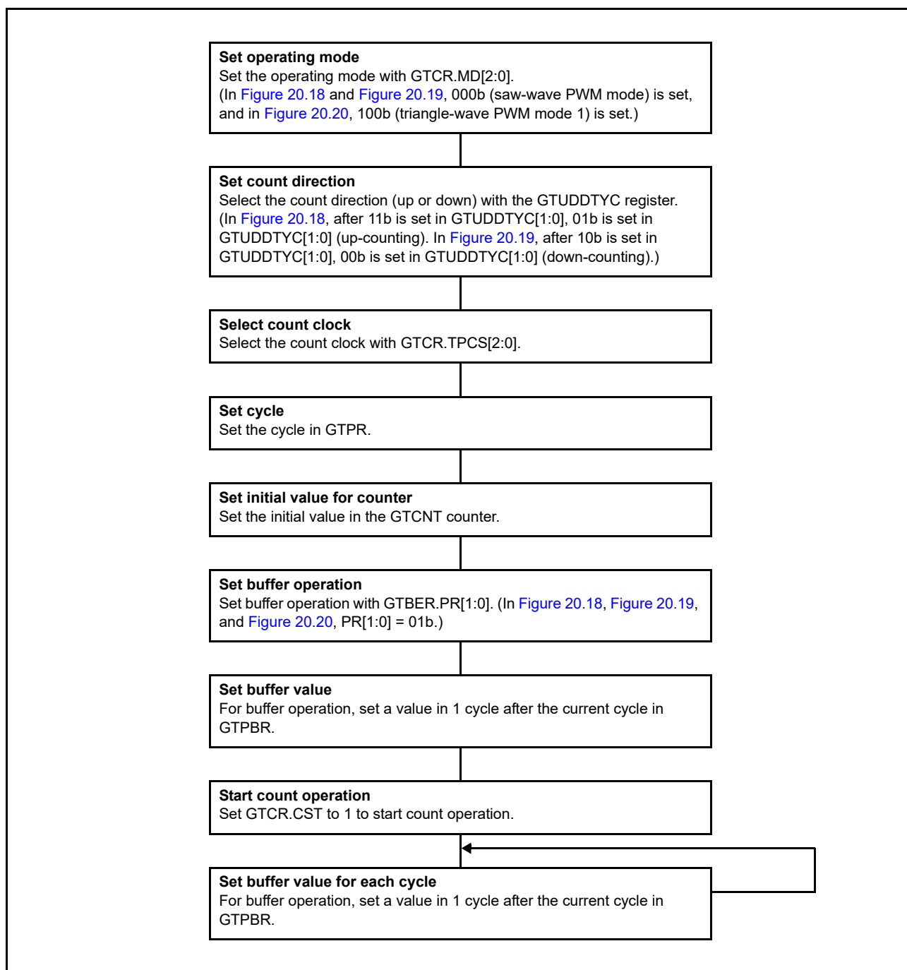
Figure 20.21 Example for setting GTPR buffer operation
