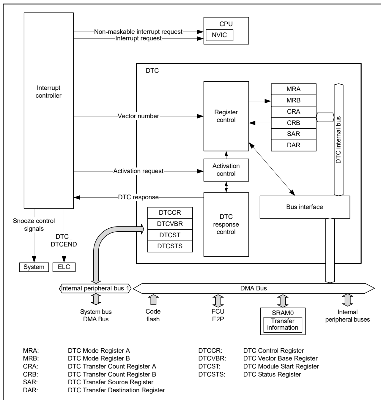
Figure 15.1 DTC block diagram
