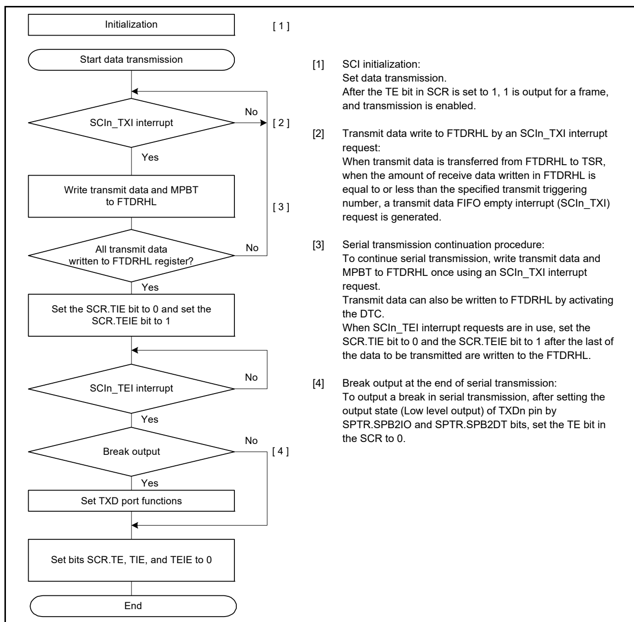
Figure 27.25 Example flow of serial transmission in multi-processor mode with FIFO selected
