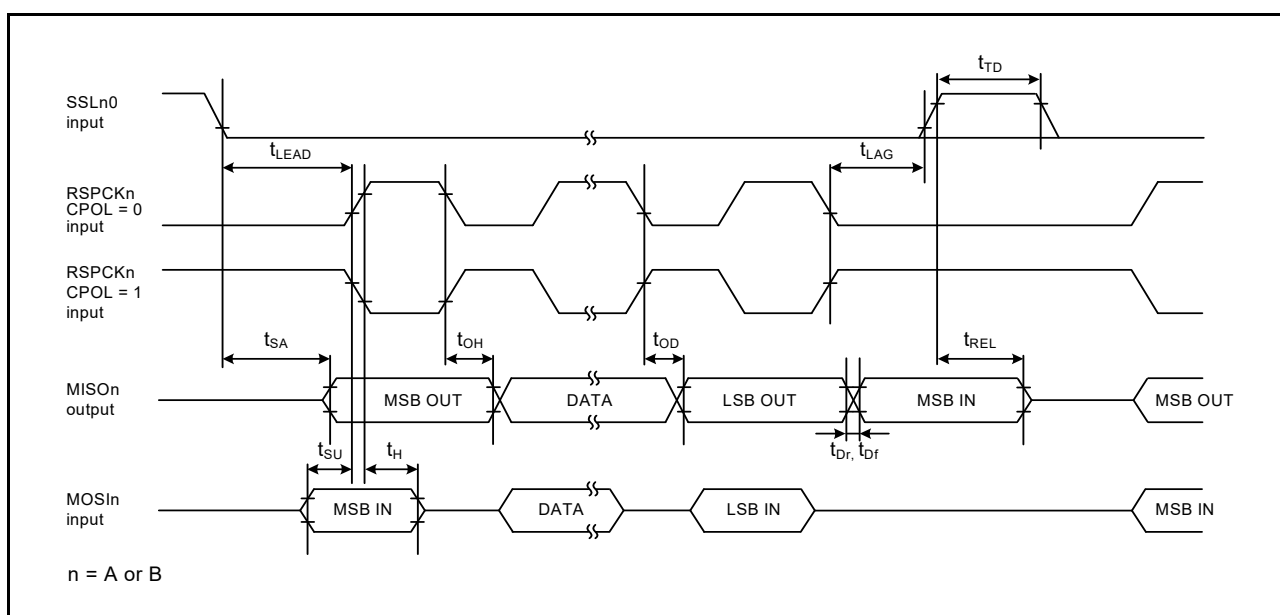
Figure 46.54 SPI timing (slave, CPHA = 0)
