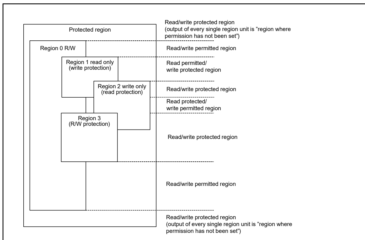
Figure 14.6 Access permission or protection by overlap of the bus master MPU regions
