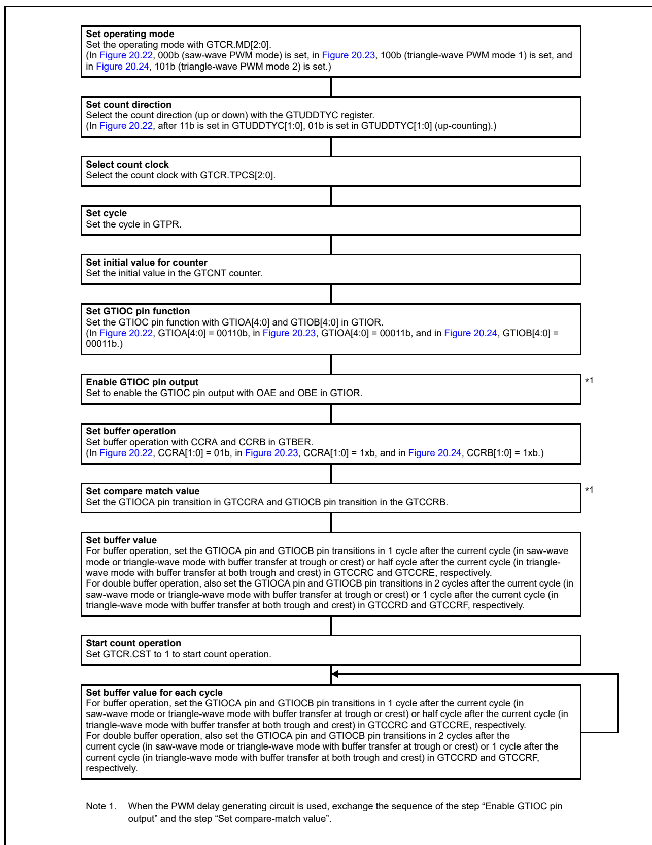
Figure 20.25 Example for setting GTCCRA and GTCCRB buffer operation for output compare
