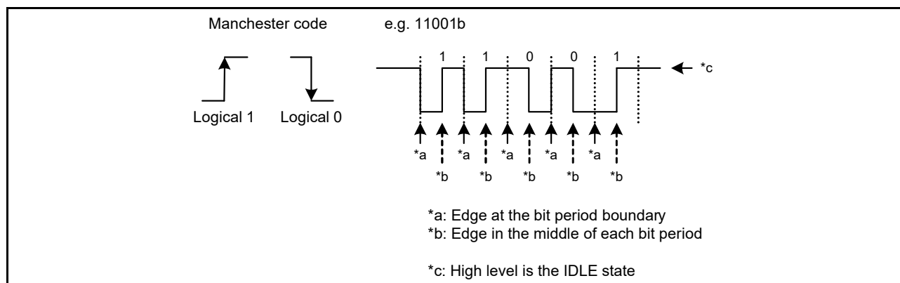
Figure 28.4 Manchester code
