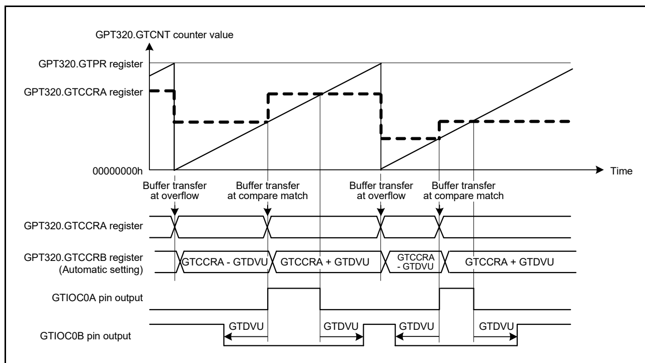
Figure 20.39 Example of automatic dead time setting function operation in saw-wave one-shot pulse mode, up-counting, and active-high
