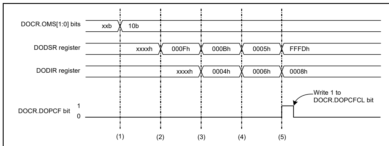
Figure 40.4 Example operation in data subtraction mode
