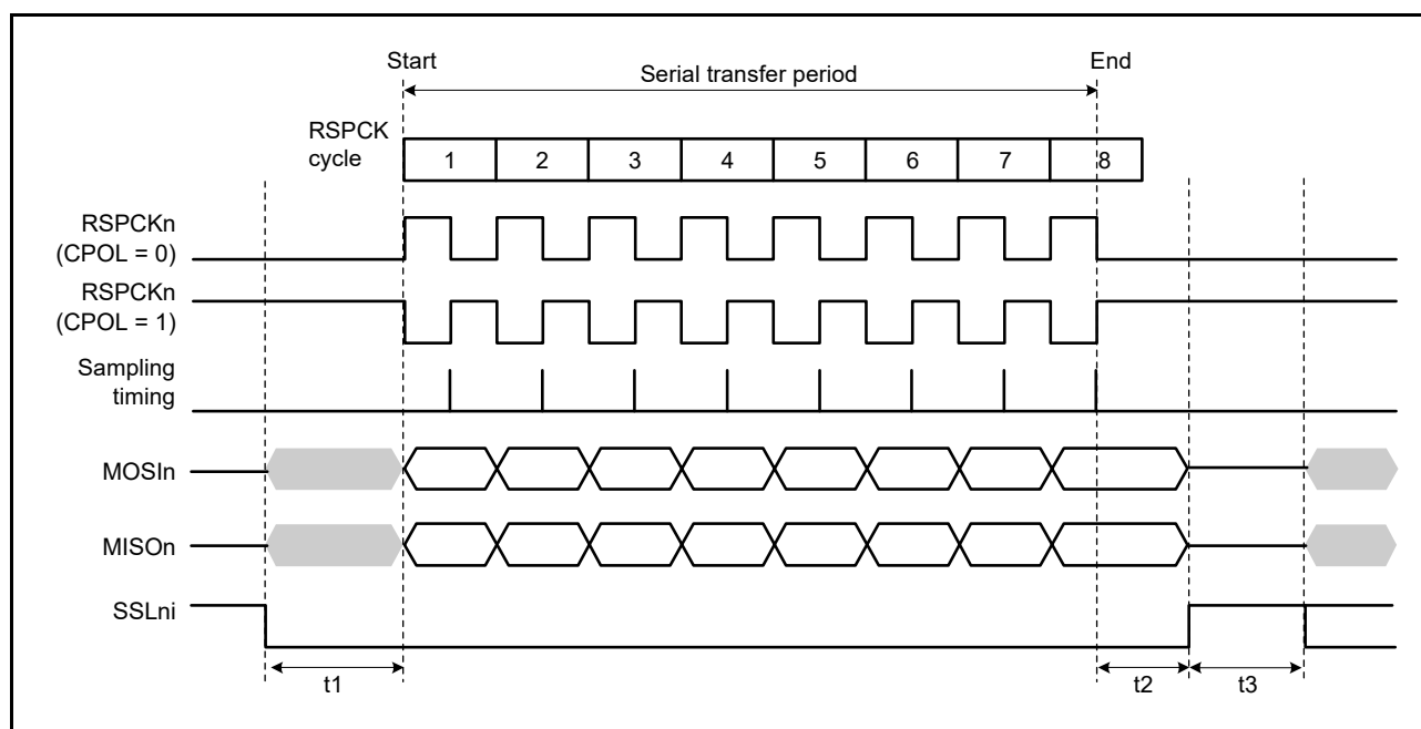
Figure 31.23 SPI transfer format when CPHA = 1
