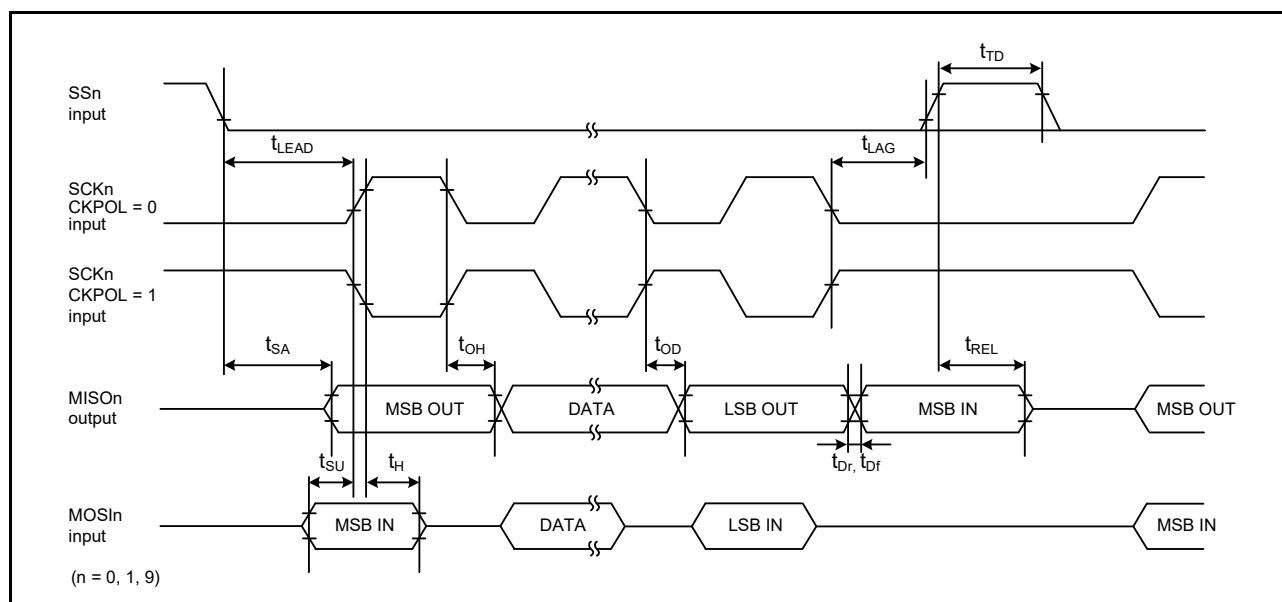
Figure 46.46 SCl simple SPI mode timing (slave, CKPH = 1)
